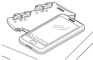
Figure 2 Connection establishment
